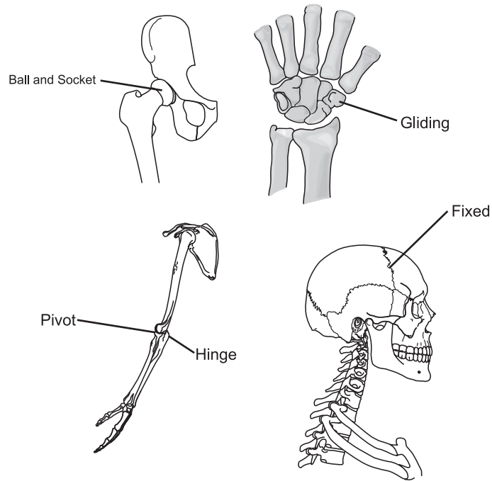
Human joints
