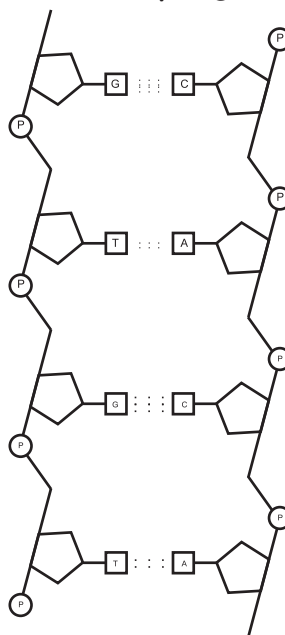
DNA base-pairing
