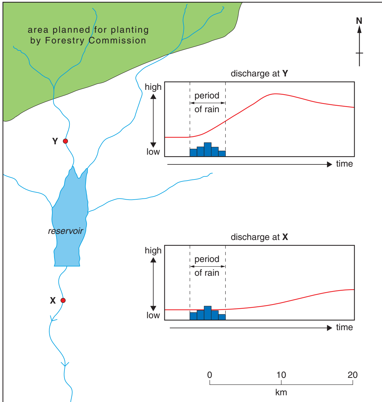
Fig. 2 Part of a drainage basin
