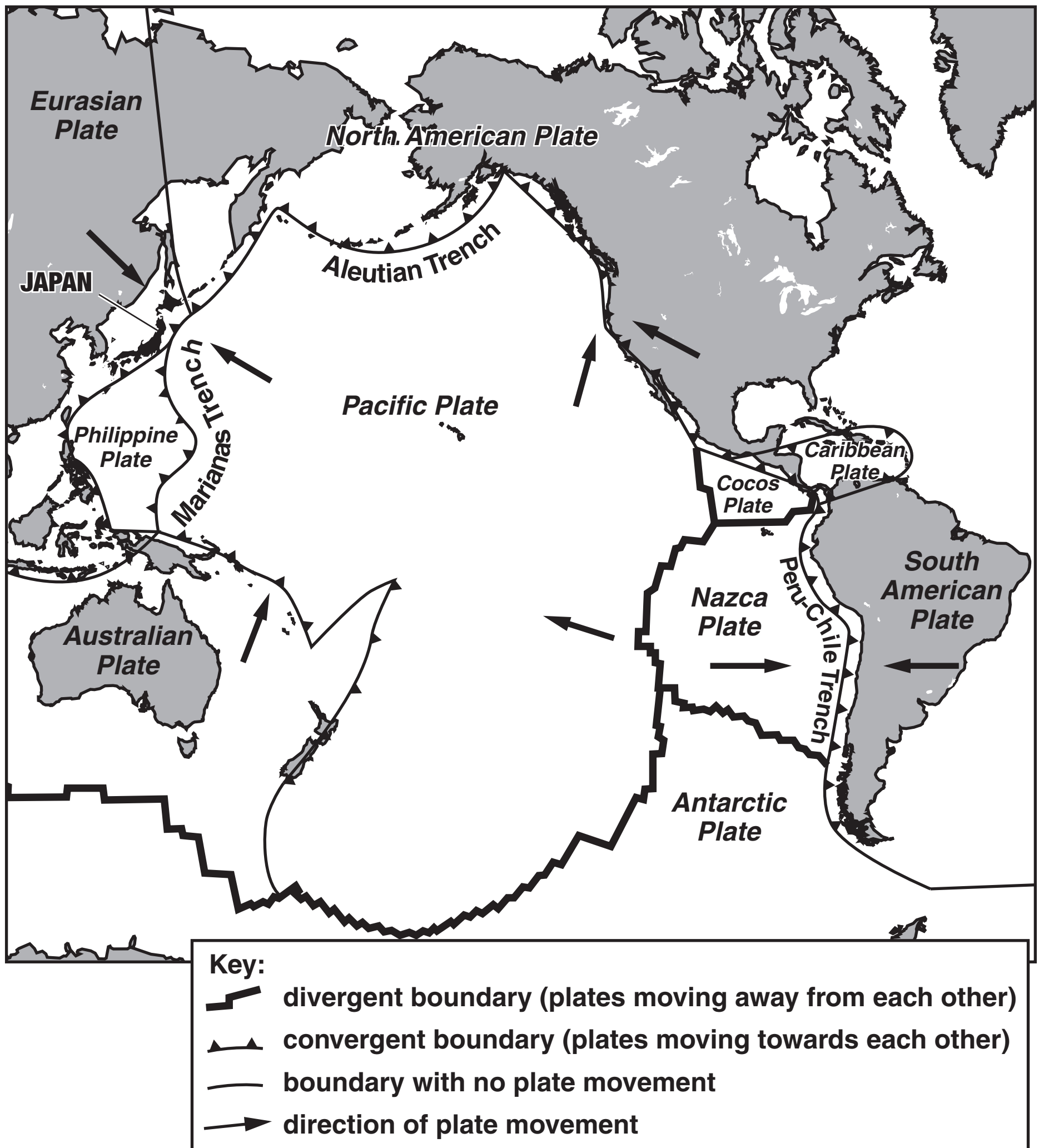
FIG. 1 MAP OF PACIFIC SHOWING PLATE BOUNDARIES
