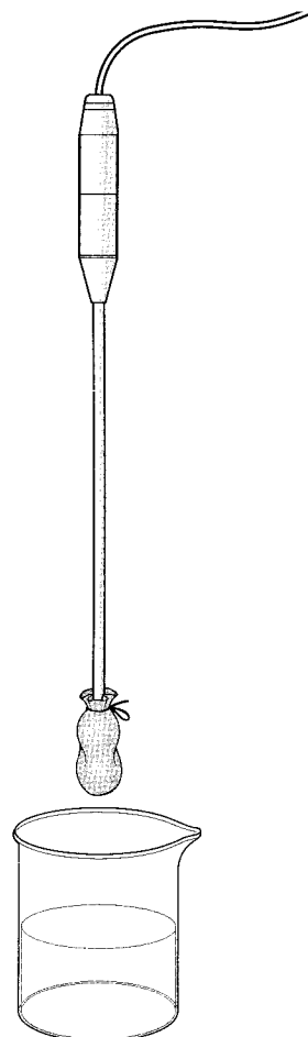
sensor R: gauze dipped in ethanol
