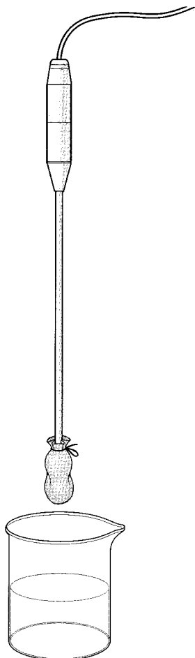
sensor Q: gauze dipped in water
